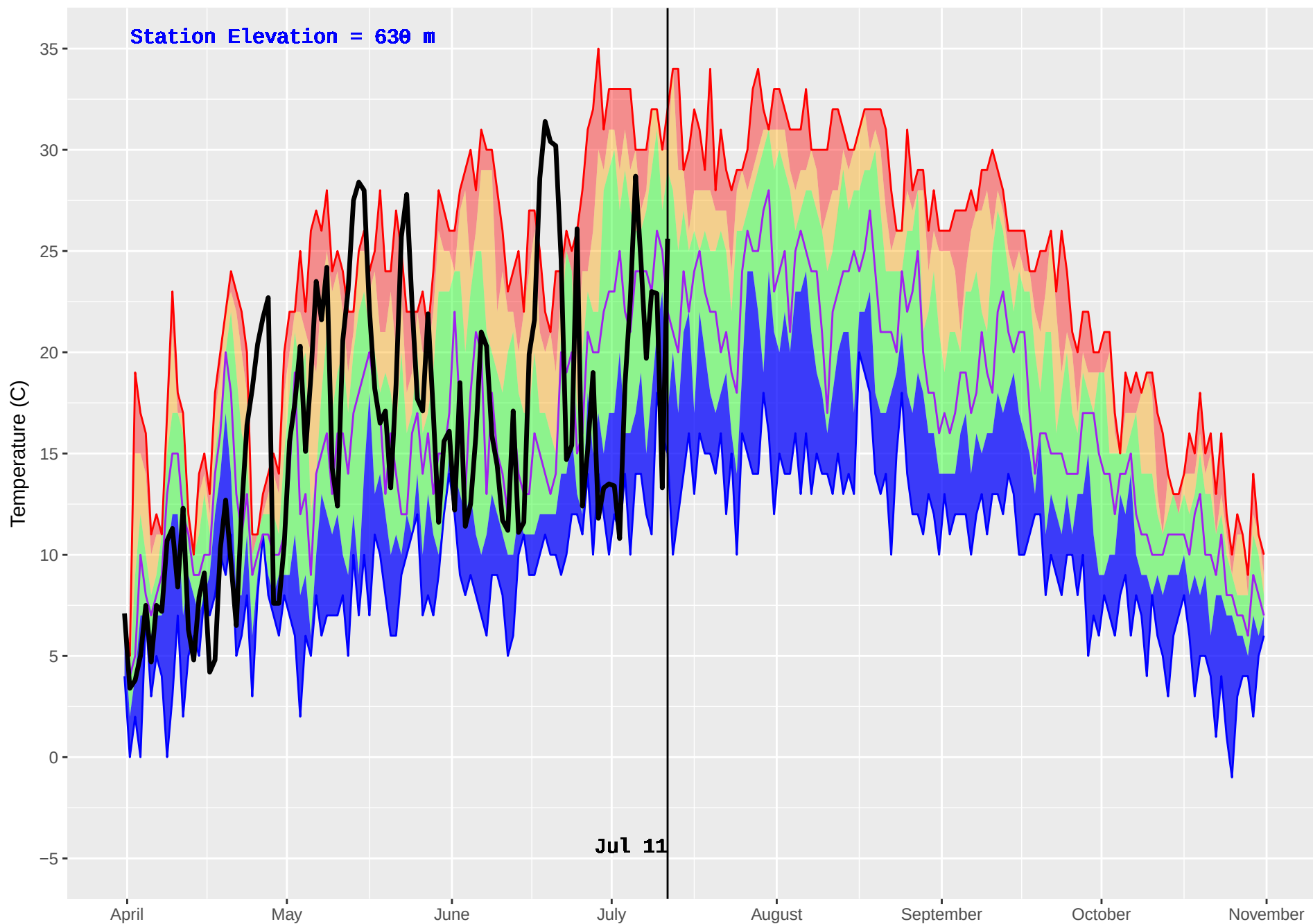
ANDERSON CREEK (977) : Historical (2007–2016) and Current (2018) Noon Temperature
