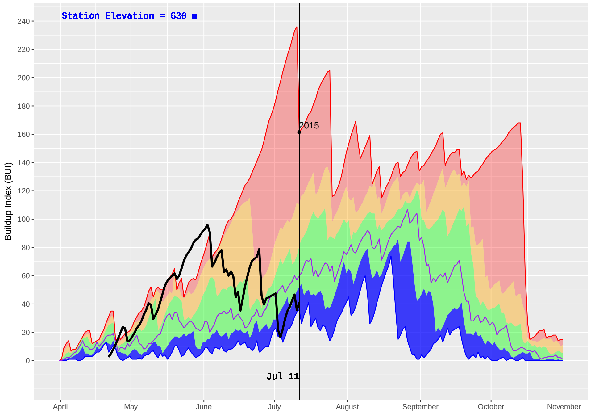
ANDERSON CREEK (977) : Historical (2007–2016) and Current (2018) Noon Buildup Index (BUI)
